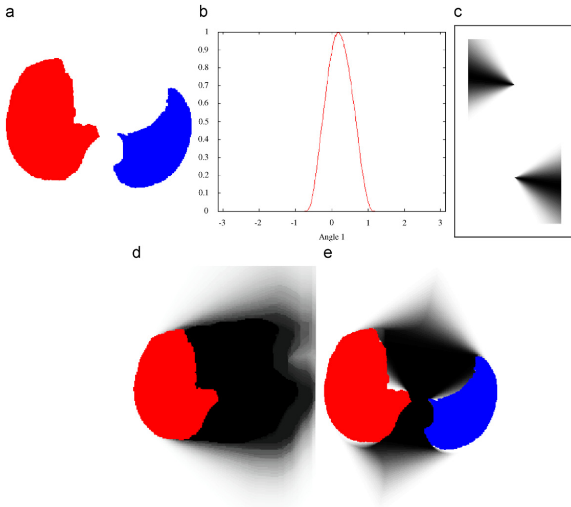
Fig. 3. Some of the steps for computing \beta_{btw}(A_1, A_2) : (a) The segmented lungs A_1 (in red) and A_2 (in blue), (b) the normalized angle histogram H_{(A_1, A_2)} with respect to the horizontal axis, (c) the structuring elements v_1 (top) and v_2 (bottom), (d) fuzzy dilation of the right lung ( A_1 ) with the fuzzy structuring element v_2 , D_{v_2}(A_1) , (e) fuzzy region \beta_{btw} between the lungs, superimposed on the segmented lungs. The membership values to \beta_{btw} vary from 0 (white) to 1 (black). The illustration is provided in 2D for the sake of readability.
